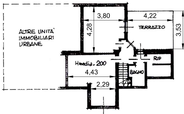
PIANTA PIANO MANSARDA
