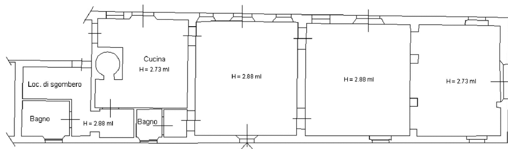
PIANO TERRA
